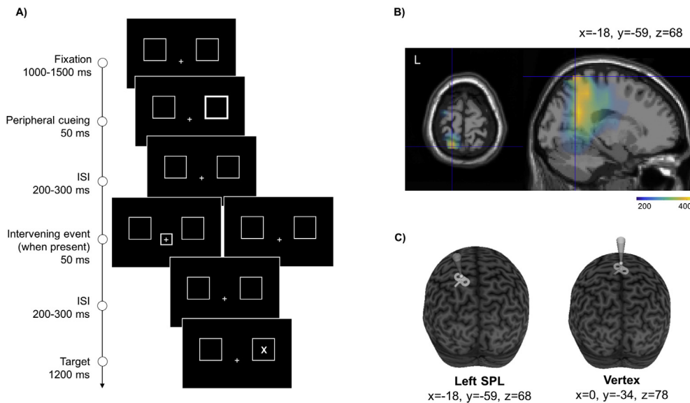
Fig. 1 – A) Sequence de events in a given trial. B) Source localization analysis from our previous EEG data (Martín-Arévalo et al., 2014) pointed to the left superior parietal gyrus/lobe (SPL) as the generator of the P1 component. In the scale, greater values (and/or warmer colors) represent greater brain activity in those areas during the P1 time window (160 msec), expressed as percent relative change respect to the baseline (pre-stimulus) period. L = Left. C) TMS stimulation site based on the source localization analysis (left part) and vertex (right part).
