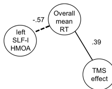
Fig. 3 – Network plot of non-zero edges for main variables in each model (EBIC graphical lasso). Model including left SLF-I HMOA, mean overall RT, and the TMS effect. Thick lines represent positive associations, while dashed lines represent negative associations. No lines represent no associations. The line thickness represents the strength of the association and numbers indicate the weight of the association.
