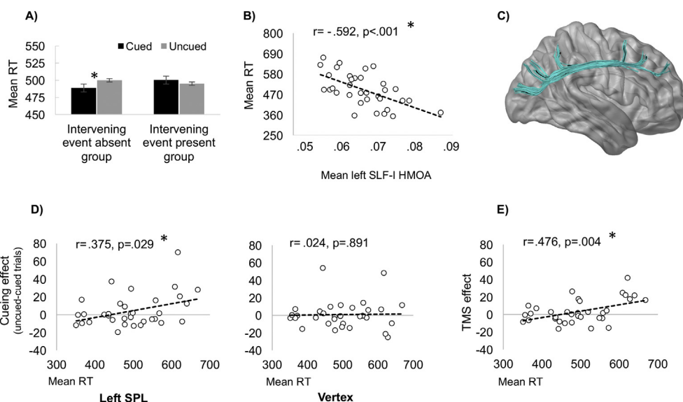
Fig. 2 – A) Mean RTs (in msec) for each experimental condition of cueing, and intervening event. Errors bars represent standard errors of the mean. B) Pearson correlation between the mean overall RT and the mean left SLF-I HMOA. C) Virtual in vivo dissection of the left SLF-I using deterministic tractography. D) Pearson correlation between the mean overall RT and the cueing effect (uncued-cued trials) for both left SPL stimulation (left part) and vertex stimulation (right part). E) Pearson correlation between the mean overall RT and the TMS effect (cueing effect on the SPL-TMS condition minus cueing effect on the vertex-TMS condition). Asterisks represent statistically significant effects.
